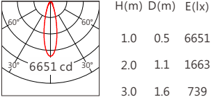
OSRAM SSL80 30° 3000K
