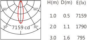
OSRAM SSL80 30° 4000K
